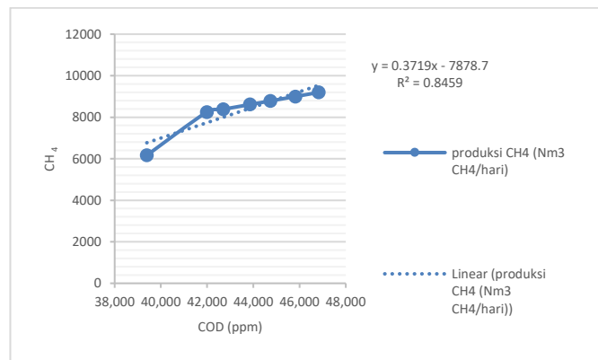
Figure 1 Linear Regression Equation of the Effect of COD on CH 4 .
