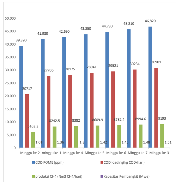
Figure 2 Estimation of Biogas Potential with a Capacity of 60 tons/hour
