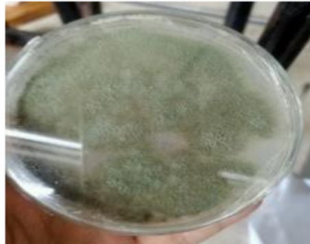
Figure 3. Misellium of Trichoderma sp.
